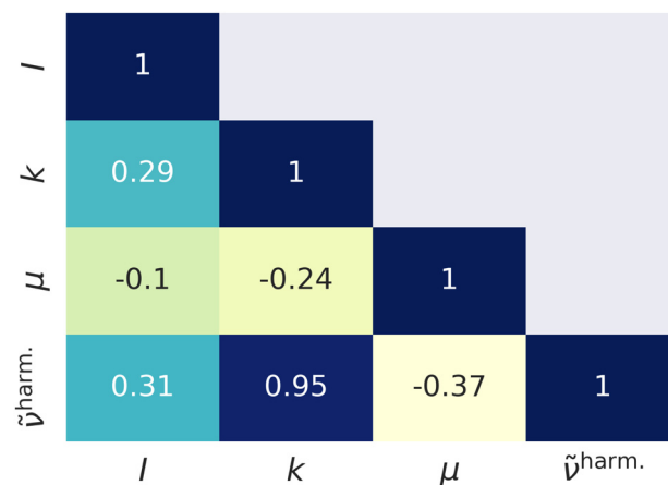
Fig. 2 Linear correlation coefficients of the descriptors. l – intensity of the harmonic vibration.
