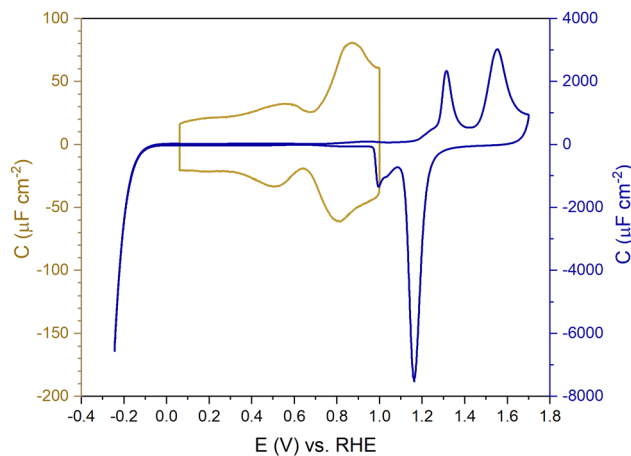
Fig. 1 Capacitance vs. potential curve showing the double-layer region (golden) and oxidation and reduction at positive potentials and HER at negative potential (blue) of Au(111) measured in Ar gas-saturated 1 mM \text{HClO}_4 solution—scan rate: 20 \text{ mV s}^{-1} .
