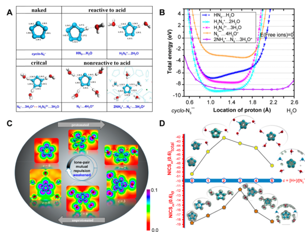
Fig. 4 (A) Optimized structures of the \text{cyclo-N}_5^- complex/crystal at various acid concentrations; (B) energetic landscape of the \text{cyclo-N}_5^- complex/crystal as a function of the N–H distance; (C) LDOS at the antibonding energy level plotted in the equatorial plane of \text{cyclo-N}_5^- under varying acidities; (D) \text{NICS}_{\text{zz}}(0.6) total and \text{NICS}_{\text{zz}}(0.6) \sigma of the \text{cyclo-N}_5^- anion under varying acidities and the corresponding LDOS isosurfaces plotted for the lowest energy level (nonbonding) of the aromatic \pi - and \sigma -systems. Reproduced with permission from ref. 90. Copyright 2019, American Chemical Society.
