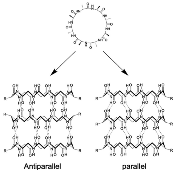
Fig. 4 Schematic illustration of the formation of antiparallel and parallel \beta -sheet structures from cyclic \alpha -alkyl peptides.
