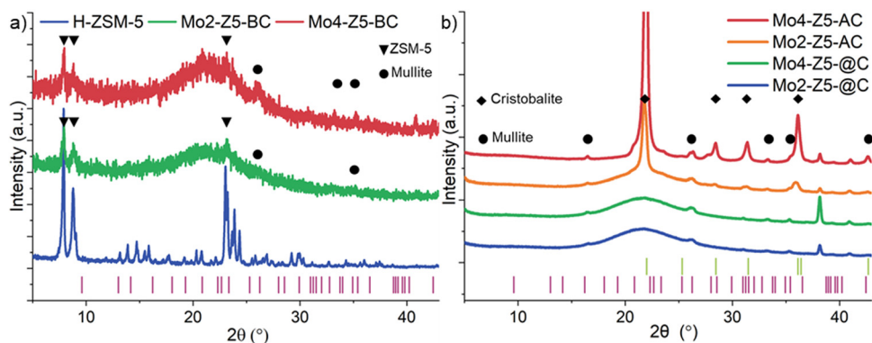
Fig. 5 PXRD patterns of Mo4-Z5-BC, and Mo2-Z5-BC compared to that of H-ZSM-5 (a), and Mo4-Z5-@C, Mo2-Z5-@C, Mo4-Z5-AC and Mo2-Z5-AC (b). Indexing lines show position reflections from the mullite (purple) and cristobalite (light green).
