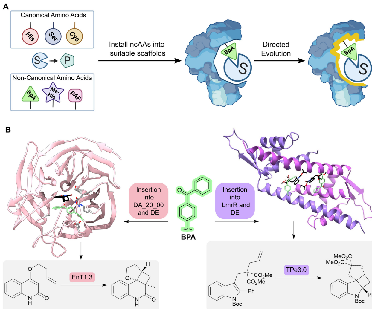
Fig. 6 Designing enzymes with non-canonical amino acids. (A) For some reactions, there may not be a natural amino acid which can act as a catalytic residue to conduct the desired chemical transformation from substrate (S) to product (P). However, some non-canonical amino acids (ncAAs) may be able to catalyze the desired transformation; these residues can be embedded into a protein scaffold to access new chemistries. However, ncAA-containing enzymes often need to be optimized further by directed evolution. (B) Using an expanded genetic code enabled the creation of enzymes for triplet energy transfer photocatalysis, unlocking new reactivity in organic synthesis. By introducing a 4-benzoylphenylalanine (BpA, green sticks) as a non-canonical photosensitizer into the Diels–Alderase DA_20_00, an enantioselective photoenzyme for thermally forbidden [2 + 2]-cycloadditions was developed (EnT1.0). The enzyme was further optimized by directed evolution to give EnT1.3 (pink ribbon, PDB: 7ZP7, product of reaction represented as atom coloured sticks with black carbons, mutations highlighted as light grey sticks). Embedding of the same ncAA (BPA, green sticks) into a different scaffold, LmrR, allowed the development of a photoenzyme for intramolecular [2 + 2] photocycloadditions of N -substituted indole derivatives (Tpe). Tpe was further engineered by directed evolution to produce the most active variant TP3.0 (PDB: 7XUQ, shown as a purple ribbon, with the product of the reaction represented as atom coloured sticks with black carbons).
