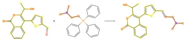
Fig. 10 Reaction for case study 2 – molecule obtained from USPTO-50k test database.
