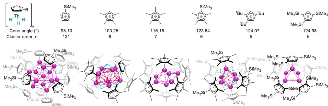
Fig. 20 Cluster order decreases with increasing with cyclopentadienyl ligand cone angle, measured from solid state structures. * The Cp' ligand results in a complex cluster of the form \{(\text{Cp}'\text{Th})_3(\text{H})_{10}\}_4\text{Th} in which the position of the hydrides is unknown. Despite its non-standard nature it is clear that this ligand can, and does, facilitate for formation of higher-order clusters than its smaller analogues. This cluster is also reminiscent of the structure of binary hydride \text{Th}_4\text{H}_{15} .
