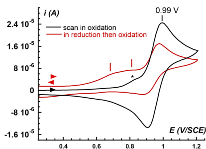
Fig. 4 CV of 1 at a concentration of 1.6 mM in \text{O}_2 saturated dry \text{CH}_3\text{CN} (at room temperature and a scan rate of 0.1 V \text{s}^{-1} ). The sample has been scanned first toward anodic potentials (black line) or first toward cathodic potential, below the reduction of \text{O}_2 ( -1.2 V) before scanning back toward anodic potentials (red line). The asterisk indicates a small amount of [\text{Fe}^{\text{II}}(\text{L}_5^2)(\text{OH}_2)]^{2+} due to the presence of residual water.
