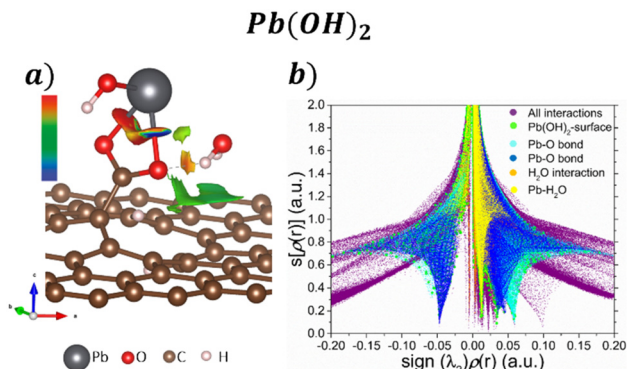
Fig. 6 a) NCI isosurface with s = 0.05 a.u. and b) s[\rho(r)] vs. \text{sign}(\lambda_2)\rho(r) graph for the adsorption \text{Pb}(\text{OH})_2 on the GO surface.
