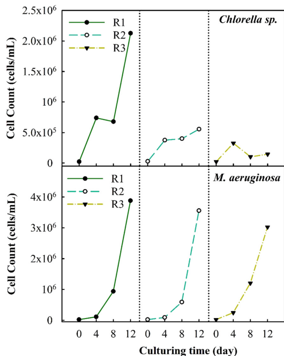
Fig. 2 Cell count of Chlorella sp. and M. aeruginosa during three rounds of cyclic culturing.
