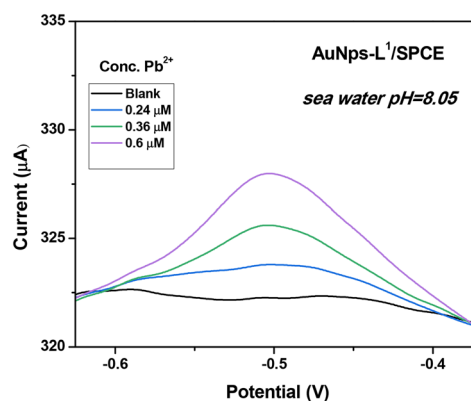
Fig. 13 Square-wave anodic stripping voltammograms (SWAVS) in seawater. Conditions: t_{\text{dep}} = 600 s and V_{\text{dep}} = -1 V.
