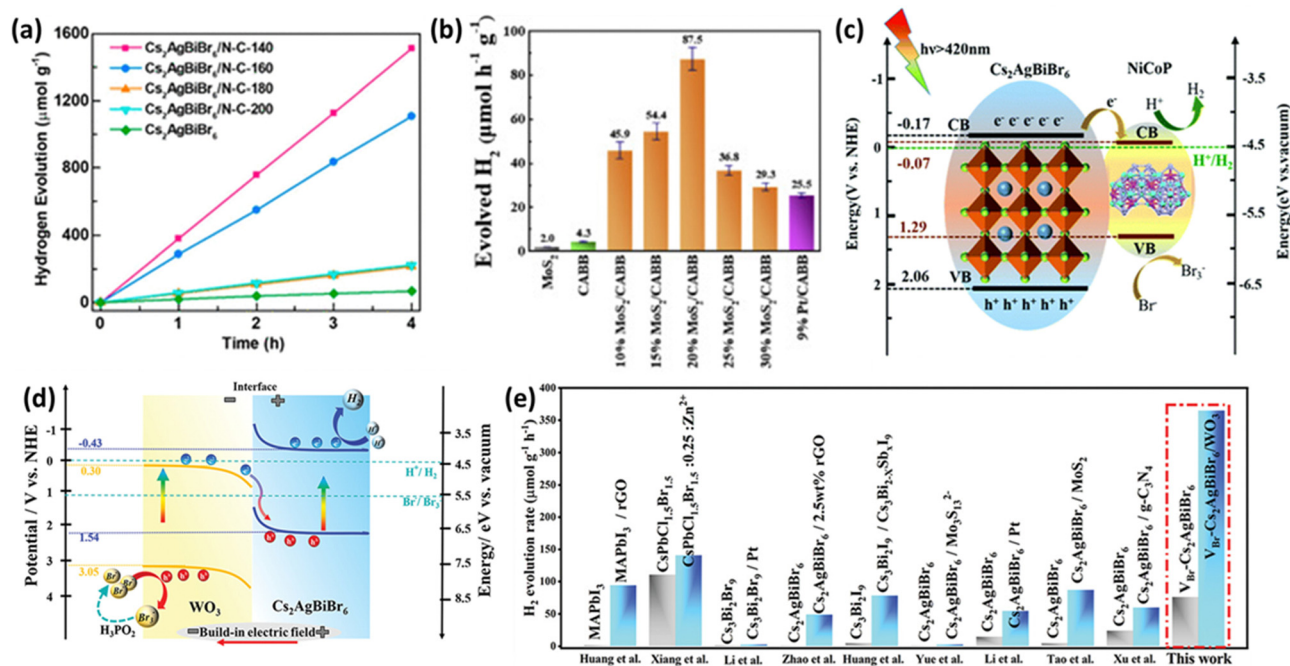
Fig. 6 (a) Hydrogen production rate from HBr aqueous solution using Cs_2AgBiBr_6 and Cs_2AgBiBr_6/N-C composites under visible light with a cutoff filter ( \lambda \geq 420 nm), and stability assessment. 91 Reproduced with permission from ref. 91 Copyright © 2021, American Chemistry Society. (b) Photocatalytic hydrogen evolution rates for MoS_2 , CABB, MoS_2/CABB , and Pt/CABB under visible light illumination ( 300 mW cm^{-2} , \lambda \geq 420 nm). 93 Reproduced with permission from ref. 93 Copyright © 2021, American Chemical Society. (c) Mechanism for photocatalytic hydrogen generation over NiCoP (NCP)/ Cs_2AgBiBr_6 (CABB). 94 Reproduced with permission from ref. 94 Copyright © 2022 Royal Society of Chemistry. (d) Schematic representation of charge transfer and dynamic equilibrium processes. (e) Comparative analysis of hydrogen evolution performance between previously reported perovskite-based catalysts and VBr-Cs_2AgBiBr_6/WO_3 . 98 Reproduced with permission from ref. 98 Copyright © 2023 Wiley-VCH GmbH.
