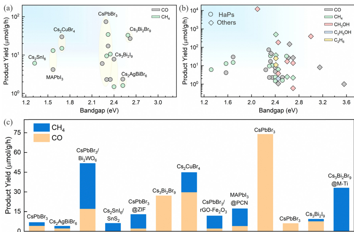
Fig. 8 (a) Product yield during photocatalytic \text{CO}_2 reduction for various perovskites, (b) comparison of products and their respective yield for HaPs and other semiconductors, 16,131,154–166 and (c) product distribution from different perovskites and perovskite heterojunctions. 13,93–101,109,111,144
