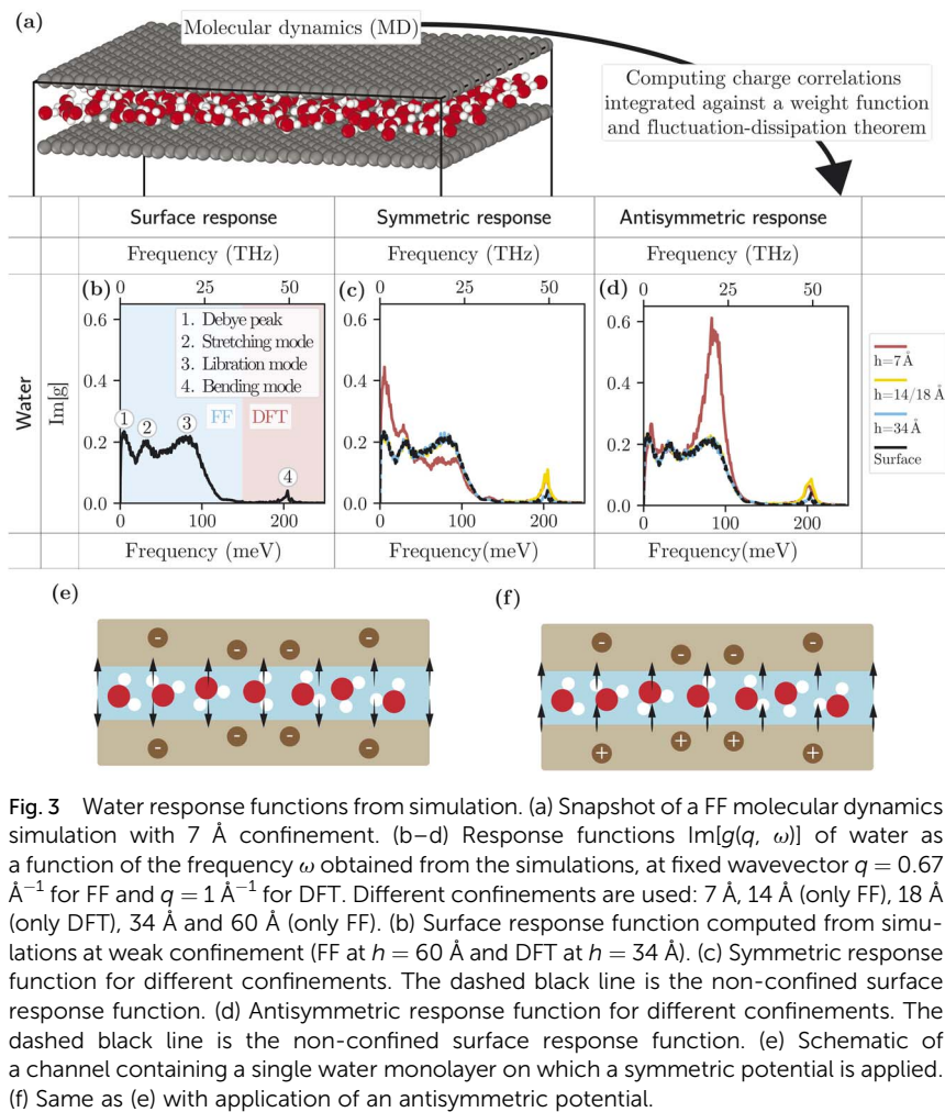
Fig. 3 Water response functions from simulation. (a) Snapshot of a FF molecular dynamics simulation with 7 Å confinement. (b–d) Response functions \text{Im}[g(q, \omega)] of water as a function of the frequency \omega obtained from the simulations, at fixed wavevector q = 0.67 \text{ \AA}^{-1} for FF and q = 1 \text{ \AA}^{-1} for DFT. Different confinements are used: 7 Å, 14 Å (only FF), 18 Å (only DFT), 34 Å and 60 Å (only FF). (b) Surface response function computed from simulations at weak confinement (FF at h = 60 \text{ \AA} and DFT at h = 34 \text{ \AA} ). (c) Symmetric response function for different confinements. The dashed black line is the non-confined surface response function. (d) Antisymmetric response function for different confinements. The dashed black line is the non-confined surface response function. (e) Schematic of a channel containing a single water monolayer on which a symmetric potential is applied. (f) Same as (e) with application of an antisymmetric potential.
