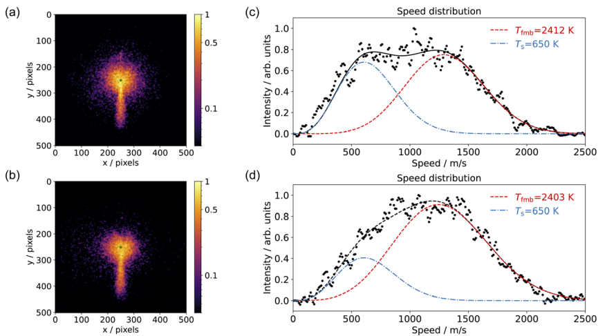
Fig. 4 Comparison of the velocity-map images of CO 2 from CO oxidation on Pd(110) at T_s = 650 K and (a) a pure CO beam with p_{\text{CO}_2} = 7.5 \times 10^{-8} mbar; (b) a 10% O 2 in He beam with p_{\text{CO}} = 5 \times 10^{-6} mbar in the scattering chamber. The green dot in (a) and (b) represents the center of the image (zero velocity). (c) and (d) show the corresponding speed distributions (black dots) for CO 2 from (a) and (b), respectively. The speed distribution is fitted (black dashed) with one slow component (blue dashes) and one fast component (red dashes).
