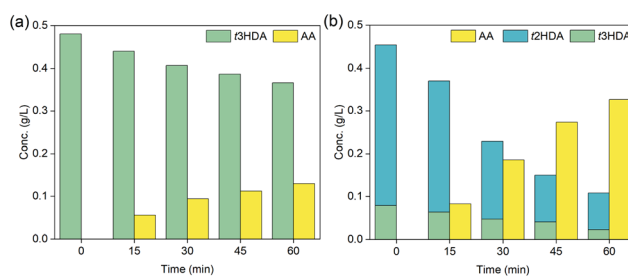
Fig. 5 Concentration ( g L^{-1} ) of trans -2-hexenedioic acid (t2HDA), trans -3-hexenedioic acid (t3HDA) and adipic acid (AA) with reaction time (min) for constant-current ( -100 mA) bulk electrolysis using (a) t3HDA, and (b) HDA mix model solutions on Pd/C.
