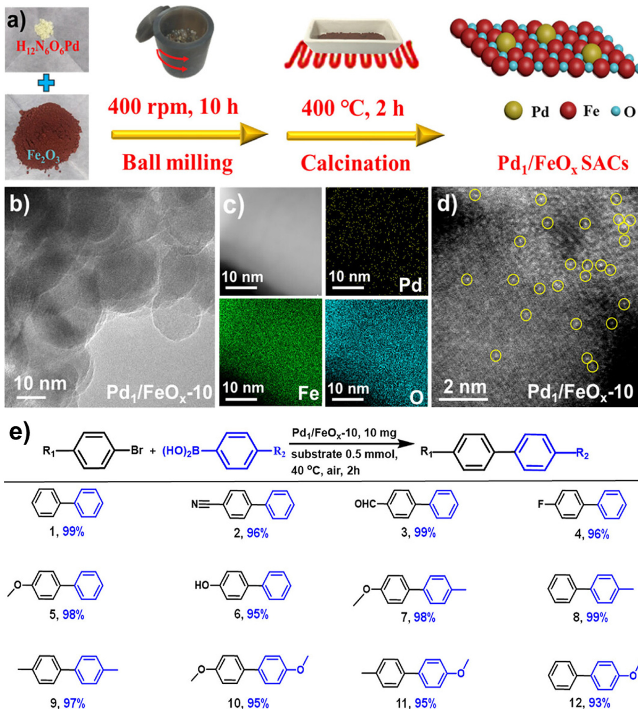
Fig. 5 (a) Schematic representation of the synthesis of Pd 1 /FeO x -10 catalysts; TEM (b), elemental mapping (c) and AC HAADF-STEM (d) images of Pd 1 /FeO x -10; (e) Pd 1 /FeO x -10 catalyzed Suzuki–Miyaura cross-coupling. Reproduced with permission from ref. 126 Copyright 2022, American Chemical Society.
