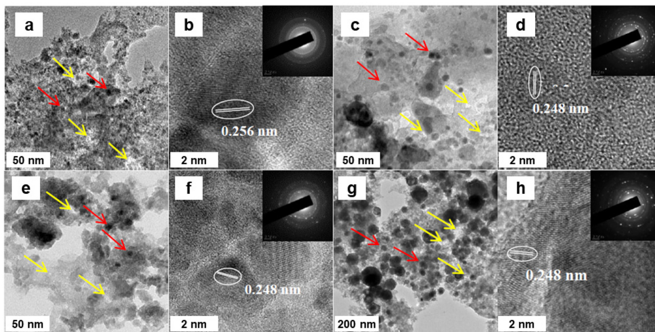
Fig. 67 TEM images of (a, b) \text{Fe}_3\text{O}_4@\text{amC}_{350} , (c, d) \text{Fe}_3\text{O}_4@\text{amC}_{550} , (e, f) \text{Fe}_3\text{O}_4@\text{amC}_{700} , and (g, h) \text{Fe}_3\text{O}_4@\text{amC}_{900} nanocomposites (insets: corresponding SAED patterns). Reproduced with permission from ref. 424 Copyright 2013, The Royal Society of Chemistry.
