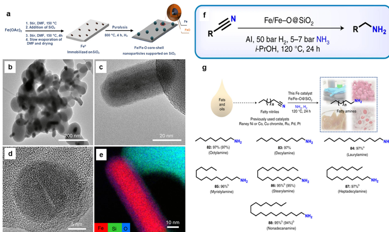
Fig. 19 (a) Schematic representation for the preparation of Fe/Fe-O core-shell NPs; (b, c) TEM; (d) HR-TEM images of \text{Fe}(\text{OAc})_2\text{-SiO}_2\text{-800} ; (e) Elemental mapping image of Fe, Si and O; (f) Application of the catalyst for the various nitrile hydrogenation; and (g) Reduction of fatty nitriles. Reproduced with permission from ref. 170 Copyright 2021, Springer Nature.
