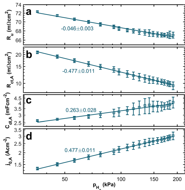
Fig. 6 Double-logarithmic plots of (a) the uncompensated resistance; (b) the charge transfer resistance at the anode; (c) the double-layer capacitance of the anode; and (d) the effective exchange current density of the HOR. All against the hydrogen partial pressure.
