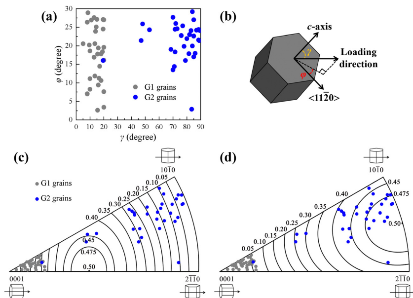
Fig. 3 (a) \gamma and \phi angle distributions of G1 and G2 grains. (b) Schematic diagram of \gamma and \phi angles. (c) and (d) Crystallographic orientations of G1 and G2 grains, plotted on the IPF map with contours of the (c) basal Schmid factor and (d) prismatic Schmid factor.
