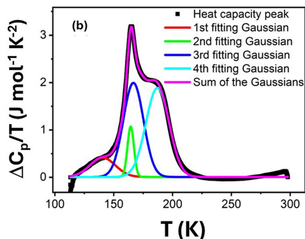
Fig. 7 (a) Heat capacity thermal profile in cooling and warming modes of 1 recorded at a scan rate of 2 \text{ K min}^{-1} . (b) Gaussian fitting of the heat capacity excess vs. temperature, derived from panel (a) along the heating process, considering four contributions.
