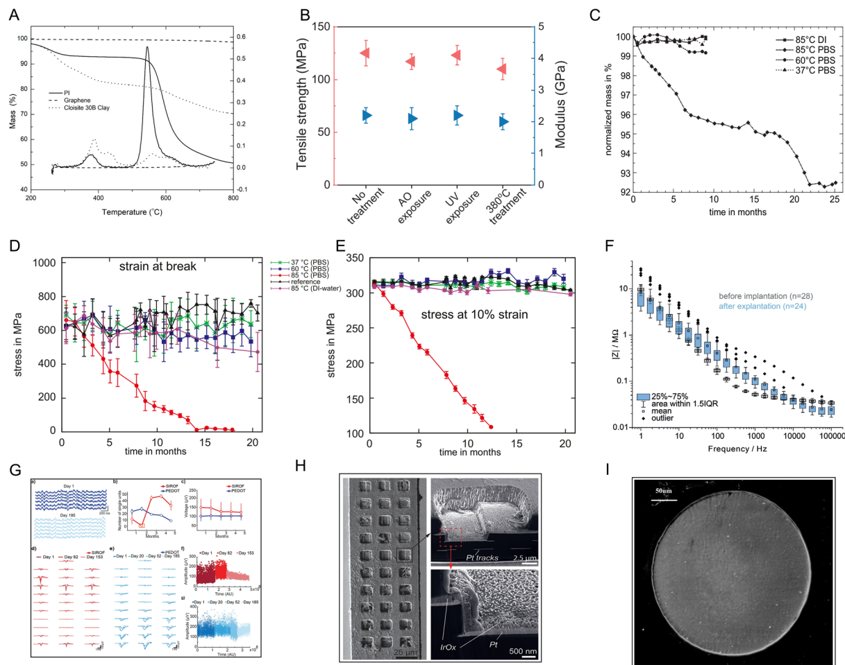
Fig. 3 Stability tests for PI. (A) TGA thermograms of neat polyimide, graphene, and Cloisite 30B clay in a nitrogen atmosphere at a heating rate of 30 °C min -1 . Reproduced with permission. 36 Copyright 2021, MDPI. (B) The tensile strength and Young's modulus of a PI–mica film change a little after AO, UV, and high-temperature exposure. Reproduced with permission. 37 Copyright 2013, WILEY-VCH. (C) The mass loss curve and (D and E) stress–strain curve of PI stored in PBS show that PI was stable in PBS at body temperature and even at 60 °C. Reproduced with permission. 38 Copyright 2010, Elsevier. (F) Electrochemical impedance spectra and (G) long-term imaging of a PI probe implanted in the mouse cortex for 180 d. (H) SEM image showing the overall intact probe with any signs of delamination or corrosion. Reproduced with permission. 40 Copyright 2023, WILEY-VCH. (I) SEM image of a microelectrode six months after its implantation in rabbit eyes shows no damage of the surface or accumulation of tissue matter. Reproduced with permission. 15 Copyright 2013, Springer Nature.
