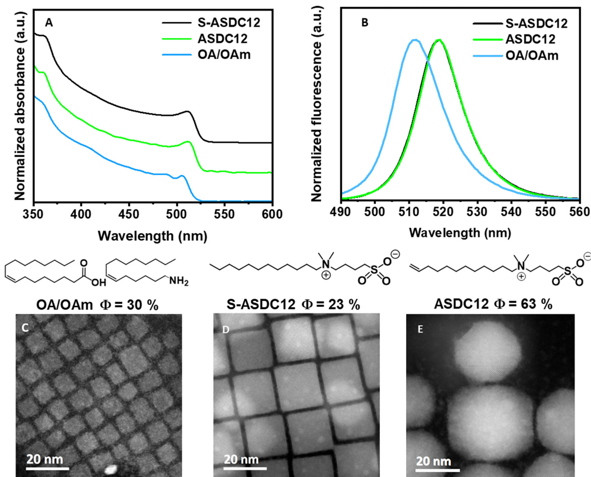
Fig. 5 Absorbance (A) and PL (B) spectra of CsPbBr 3 NCs capped with OA/OAm, and (C)–(E) HAADFpn images and their respective PLQY ( \Phi ).
