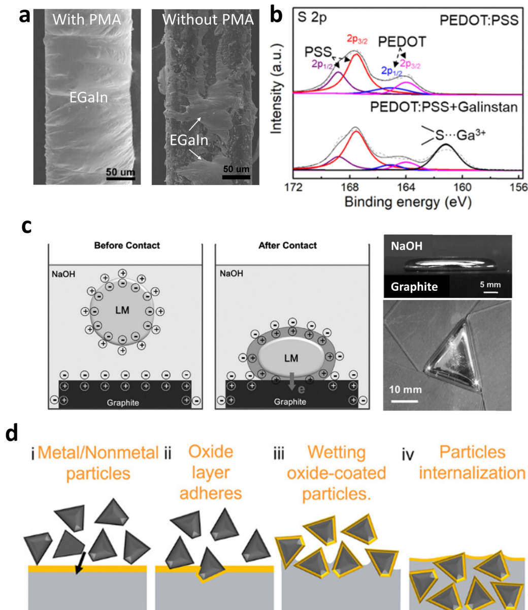
Fig. 12 Interactions of GalLMs with non-metallic materials. (a) SEM images of the conductor fiber covered by EGaln with PMA intermediate layer (left) and without PMA (right). Reproduced with permission from ref. 147 Copyright 2020 American Chemical Society. (b) S 2p XPS spectrum of PEDOT:PSS before and after mixing with Galinstan. Reproduced with permission from ref. 149 Copyright 2023 Elsevier. (c) Flattening deformation of Galinstan driven by electrochemical oxidation upon contacting with graphite in NaOH. The gallium oxide layer is formed on a Galinstan droplet due to the negative potential drop from Galinstan to graphite. Reproduced with permission from ref. 160 Copyright 2016 John Wiley and Sons. (d) Schematic showing the fabrication of GalLMs composites with carbon-based fillers. Reproduced with permission from ref. 165 Copyright American Chemical Society.
