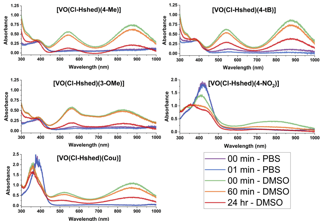
Fig. 5 UV-vis-NIR spectra of 0.10 mM catecholates complexes, recorded in both DMSO and PBS as a function of time. The complex formed with 4-CN was excluded due to low stability.
