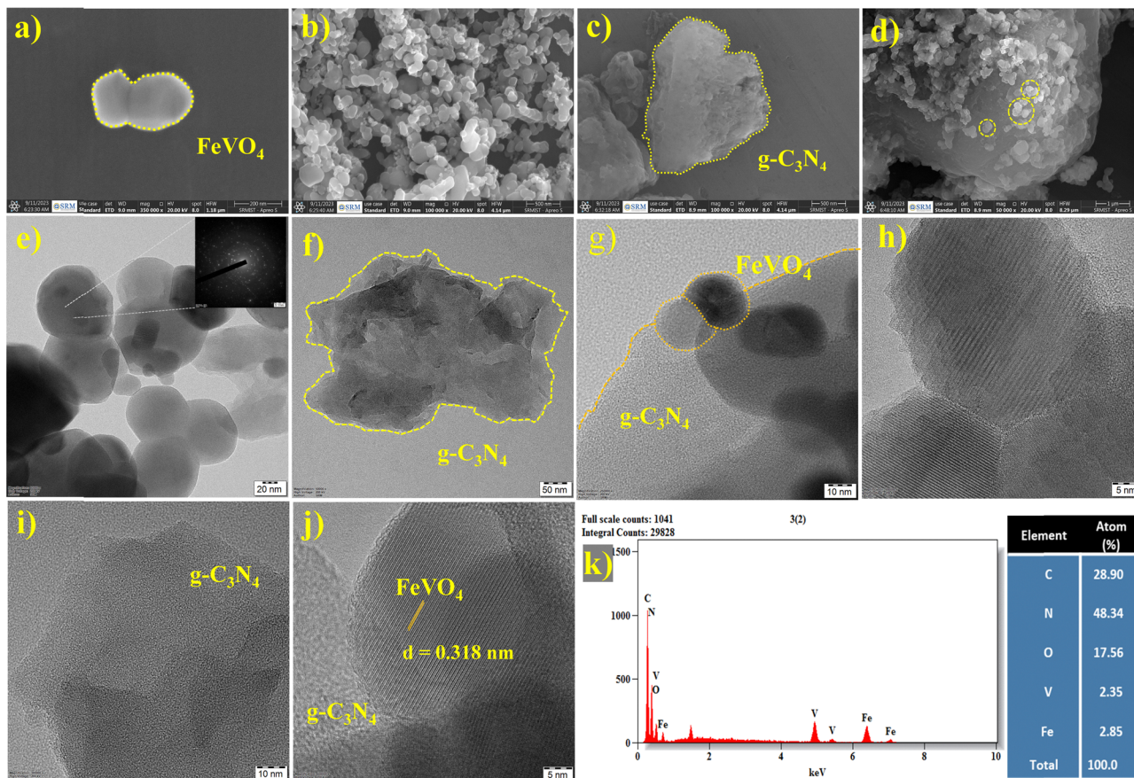
Fig. 3 SEM Micrographs of (a) and (b) FVO (FeVO 4 ), (c) CN (g-C 3 N 4 ), (d) FVO/CN, – TEM micrographs of (e)–(g) FVO, CN and FVO/CN, (h)–(j) lattice fringes of FVO, CN and FVO/CN, (k) EDX analysis of FVO/CN.
