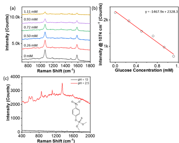
Fig. 8 (a) Glucose detection using 4-MCBA with PAA-grafted AgNPs at concentrations of 0 \text{ mM} to 1.11 \text{ mM} of glucose in addition to 0.5 \text{ M} \text{H}_3\text{PO}_4 solution. (b) Plotting the peak intensity of 4-MCBA at 1074 \text{ cm}^{-1} vs. glucose concentrations of 0 \text{ mM} to 1.11 \text{ mM} . (c) Detection of methyl parathion using PAA-grafted AgNPs at a concentration of 17 \text{ ppm} after adding \text{H}_3\text{PO}_4 .
