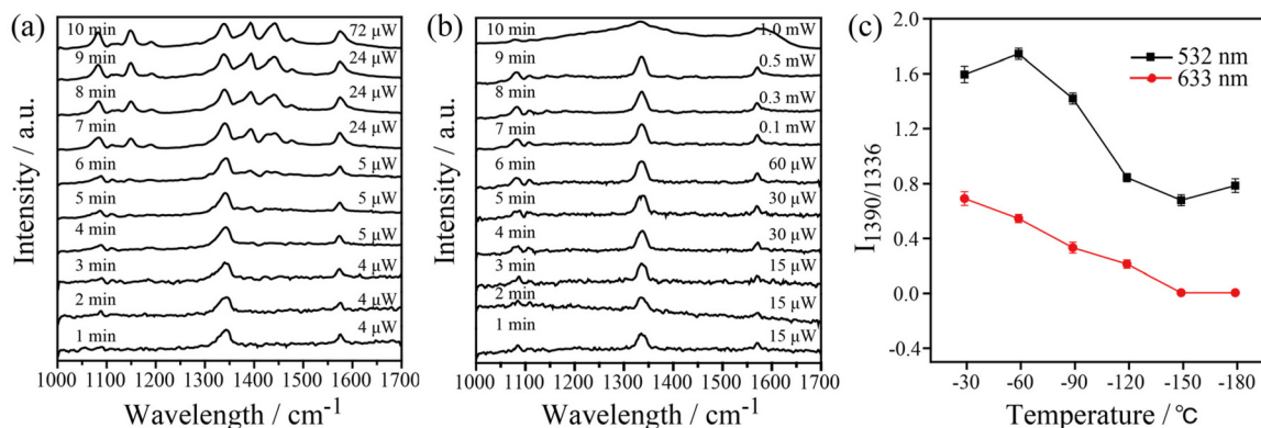
Fig. 4 Time-dependent SERS spectra of the plasmon-induced catalytic reaction of 4-NTP at -180 °C with (a) 532 nm and (b) 633 nm excitation at different laser powers on the samples. The time interval is 1 min from bottom to top, t_{\text{acq}} = 60 s; (c) the average intensity ratio of 1390 \text{cm}^{-1} /1336 \text{cm}^{-1} referring to [DMAB]/[4-NTP] as a function of temperature at 532 nm (black) and 633 nm (red).
