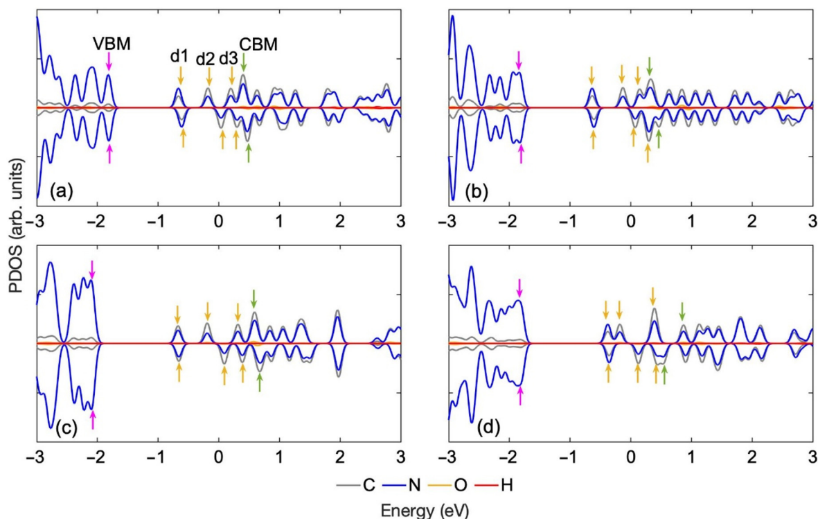
Fig. 2 Partial density of states (PDOS) for the optimized structures of the ON-GCN tautomers shown in Fig. 1: (a) NH-CN, (b) NH 3 , (c) N-H β and (d) N-H α . Hopping of just one hydrogen leads to substantial changes in the electronic properties. The Fermi level is set to 0 eV. Band edges and defect states are marked with colored arrows: VBM: pink, CBM: green, defects (d1–d3): yellow.
