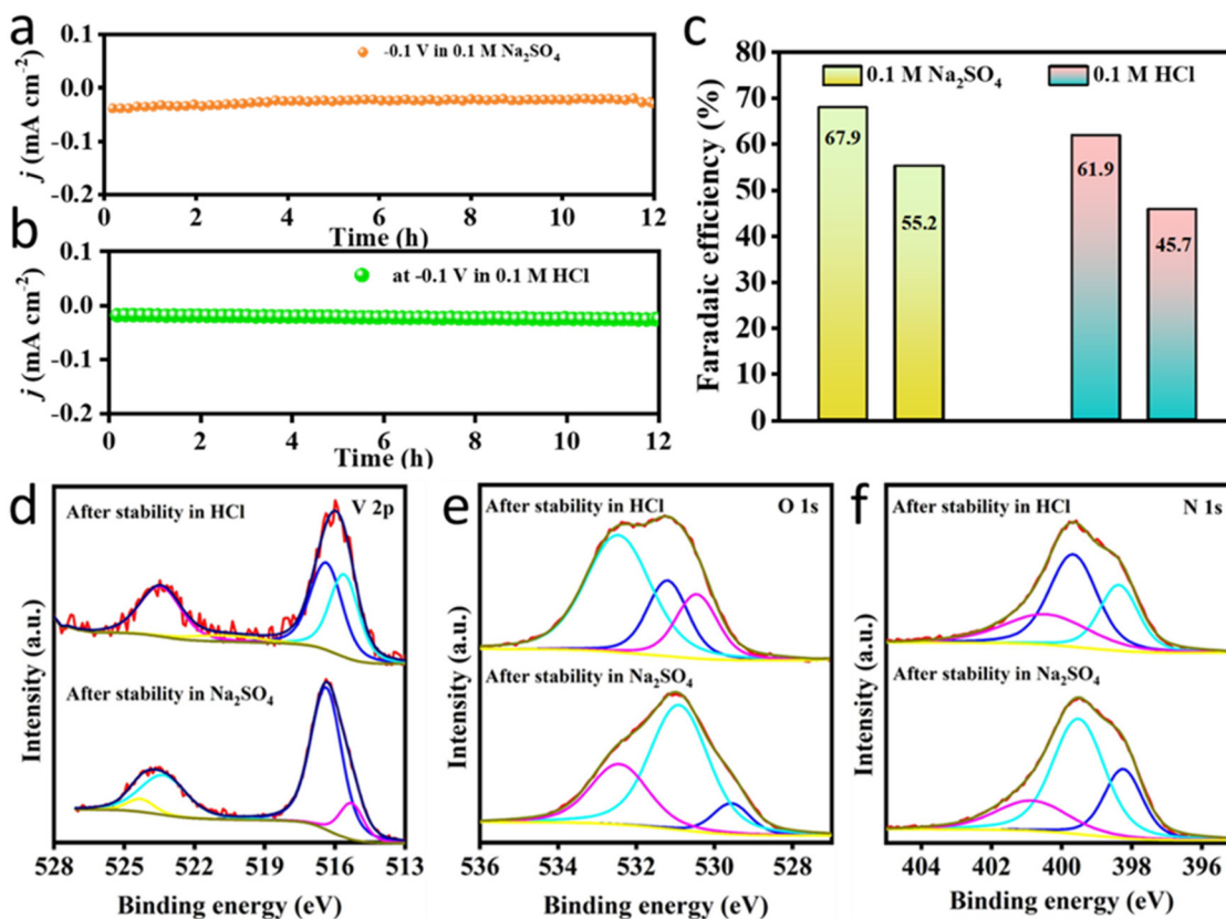
Fig. 6 (a and b) CA response of \text{VO}_2\text{@CN} during the NRR at -0.1 V vs. RHE in 0.1 M \text{Na}_2\text{SO}_4 and 0.1 M \text{HCl} , respectively, for a continuous 12 h period; (c) FE comparison of the catalyst after 1 and 12 h of NRR studies in both electrolytes; post-NRR XPS profiles for (d) V 2p, (e) O 1s and (f) N 1s, respectively, under HCl and \text{Na}_2\text{SO}_4 electrolyte conditions.
