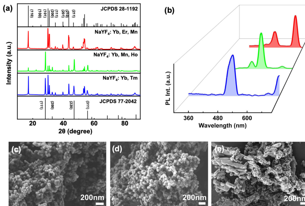
Fig. 5 (a) XRD and (b) PL plots of NaYF 4 /Yb,Tm (blue), NaYF 4 /Yb,Mn,Ho (green), and NaYF 4 /Yb,Er,Mn (red) UCNP. SEM images of (c) blue, (d) green and (e) red emitting UCNP.
