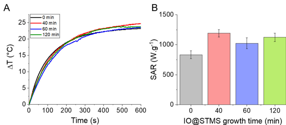
Fig. 11 (A) Temperature profiles as a function of time for the different IO@STMS- t NPs at 0.5 mgFe mL -1 under NIR light irradiation. (B) Corresponding SAR values. These results were obtained with the IO@STMS- t obtained from series 2.
