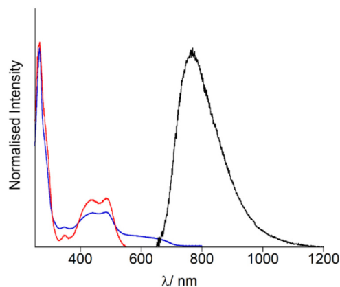
Fig. 2 Optical spectroscopy of OsPhenSS in aerated aqueous solution (2% CH 3 CN) UV-Vis absorption spectrum: blue, luminescence excitation spectrum ( \lambda_{\text{em}} = 770 nm) red, and luminescence emission spectrum ( \lambda_{\text{exc}} = 488 nm); black.
