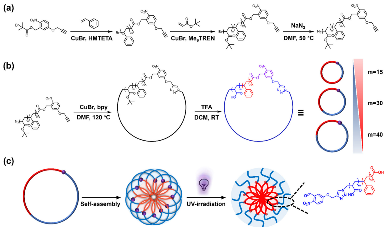
Scheme 1 (a) Synthesis of NB-PS 30 - b -PtBA m ( m = 15, 30, and 40) linear block copolymers; (b) synthesis of C-NB-PS 30 - b -PAA m cyclic block copolymers and C-NB-PS 30 - b -PAA m cyclic block copolymers; (c) schematic representation of transforming polymer assemblies with looped corona to linear corona through UV irradiation.
