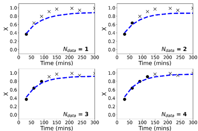
Fig. 8 Predicted evolution of conversion with time (dashed lines) for PCINN based on real-time updates with samples from reaction (8). The crosses show future, as-yet-unknown values while the circles show the measured values which are used as training data.
