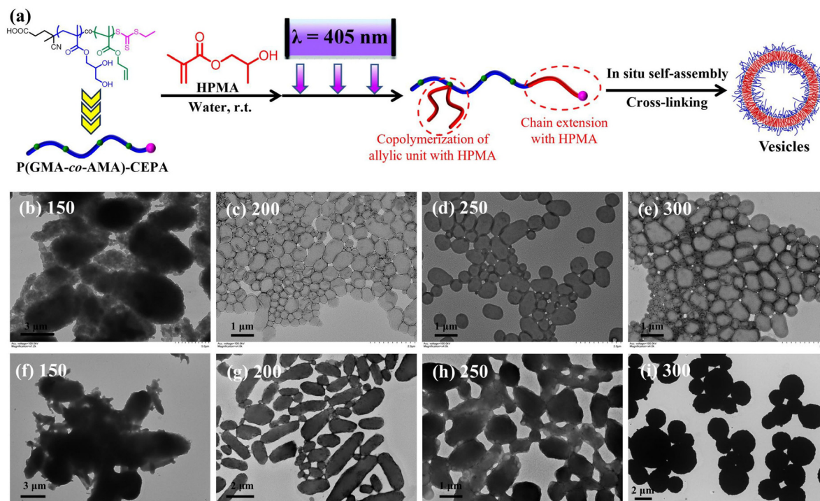
Fig. 8 (a) Schematic illustration of aqueous photoinitiated RAFT dispersion polymerization of HPMA using P(GMA 44 -co-AMA 5 )-CEPA as the macro-RAFT agent. (b–e) TEM images of polymer nanoparticles prepared by aqueous photoinitiated RAFT dispersion polymerization of HPMA (10% w/w) using P(GMA 44 -co-AMA 5 )-CEPA with different [HPMA]/[macro-RAFT] ratios. (f–i) TEM images of polymer nanoparticles prepared by aqueous photoinitiated RAFT dispersion polymerization of HPMA (20% w/w) using P(GMA 44 -co-AMA 5 )-CEPA with different [HPMA]/[macro-RAFT] ratios.
