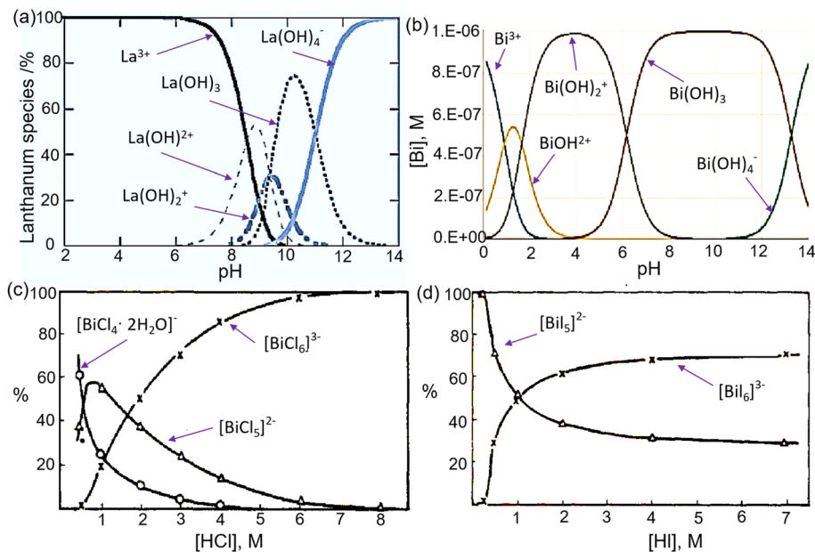
Fig. 5 Distribution species of La 3+ as a function of pH (a) (reproduced from ref. 95 with permission from the Royal Society of Chemistry, copyright 2006); distribution species of Bi 3+ (10 -6 mol L -1 ) as a function of pH (b) (reproduced (adapted) from ref. 96. with permission from the American Chemical Society, Copyright 2022); and distribution species of Bi 3+ as a function of HCl (c) and HI concentrations (d) (reproduced (adapted) from ref. 97 with permission from Elsevier, copyright 1979).
