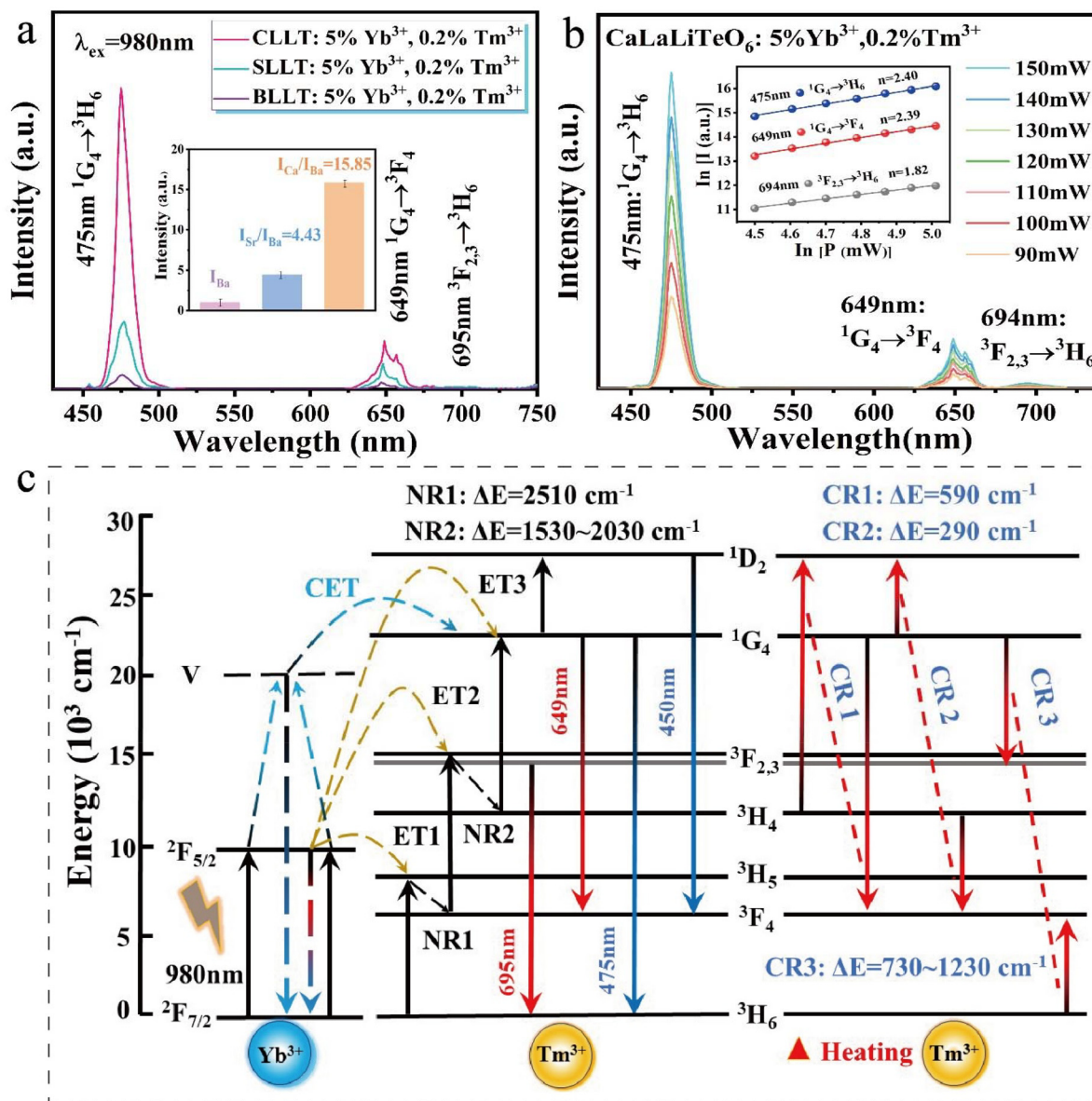
Fig. 3 (a) Up-conversion PL spectra of \text{ALaLiTeO}_6:5\%Yb^{3+},0.2\%Tm^{3+} (A = Ca, Sr, and Ba). (b) The relationship between \ln(I) and \ln(P) of \text{CaLaLiTeO}_6:5\%Yb^{3+},0.2\%Tm^{3+} . (c) Energy level diagram and thermally enhanced CR processes in the \text{ALaLiTeO}_6:5\%Yb^{3+},0.2\%Tm^{3+} phosphor.
