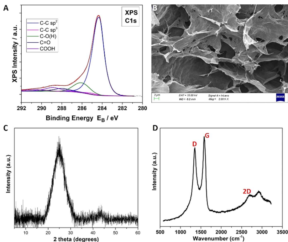
Fig. 2 Characterisation of the GO + GNPs aerogels. (A) Deconvoluted C1s XPS spectrum of the GO + GNP aerogel. (B) SEM photo of the as-obtained graphene aerogel showing the macro-porosity of the material. (C) XRD diagram of the aerogel. The as-made graphene aerogel exhibits a weak broad peak, characteristic of an amorphous material, at 2\theta = 26^\circ , which corresponds to the (002) plane of the graphite structure. (D) Raman spectrum of the aerogel showing the characteristic G, D and 2D peaks of graphene.
