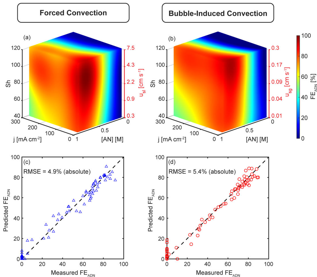
Fig. 5 (a and b) 3D GPR surrogate models showing the effect of current density ( j ), AN concentration ( [\text{AN}] ), and Sherwood number ( Sh ) on FE_{ADN} for (a) forced convection and (b) bubble-induced convection. The superficial liquid or gas velocities ( u_{sl} or u_{sg} ) corresponding to Sh are shown on the right axes in red. (c and d) Surrogate model predicted FE_{ADN} vs. measured FE_{ADN} from the forced (c) and bubble-induced (d) convection experiments. The forced convection predictions have an RMSE of 4.9% (absolute) compared to measured values and bubble-induced convection predictions have an RMSE of 5.4% (absolute) compared to measured values. All plots present predicted values from the surrogate models built on experimental data. The experiments were conducted at ambient temperature and pressure. In addition to AN, the electrolyte contained 0.5 M \text{Na}_3\text{PO}_4 , 0.03 M EDTA, and 0.02 M TBA hydroxide.
