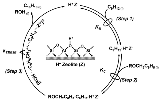
Scheme 2 Proposed reaction mechanism (via the concerted pathway) for benzylation of mesitylene (C 9 H 12 ) with a benzylating agent (ROCH 2 C 6 H 5 ) on a Brønsted acid site (H + Z - ) to form 1,3,5-trimethyl-2-benzylbenzene (C 16 H 18 ) and a leaving group (ROH). Steps are described in the text.
