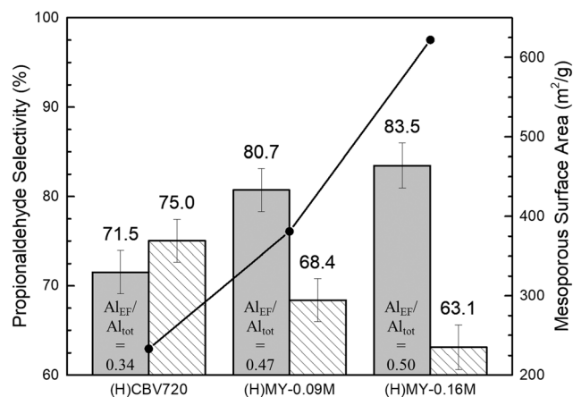
Fig. 4 (Bar graph) Propionaldehyde selectivity changes over (line plot) mesoporous surface area and Al_{EF} content of measured catalysts. (Grey) Selectivity of propionaldehyde measured with catalyst that underwent pretreatment, (dashed pattern) selectivity of propionaldehyde measured with catalyst that had no pretreatment materials, (numbers inside the bar graph) Al_{EF} content of measured catalysts. Original reaction setup conducted at 450 °C, 1 : 1 : PPG : catalyst ratio, 425 Da MW PPG polymer with 10-minute reaction time, under N_2 atmosphere.
