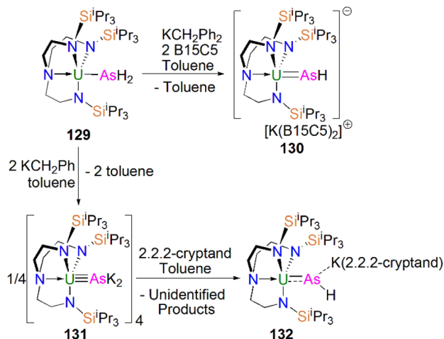
Scheme 43 Synthesis of the uranium arsenidene complexes 130 , arsenido 131 , and arseniide 132 from the arsenide 129 .
