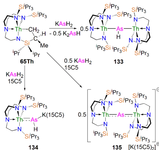
Scheme 44 Synthesis of thorium arseniide and arsenido complexes 133–135 .
