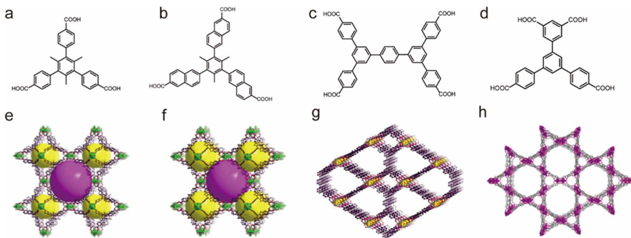
Fig. 4 The structures of the BUT series and the used ligands. (a) The H 3 CTTA ligand. (b) The H 3 TTNA ligand. (c) The BCQD ligand. (d) The H 4 CPTTA ligand. (e) BUT-12. Reproduced from ref. 93 with permission from the American Chemical Society, Copyright 2016. (f) BUT-13. Reproduced from ref. 93 with permission from the American Chemical Society, Copyright 2016. (g) BUT-14. Reproduced from ref. 94 with permission from the American Chemical Society, Copyright 2017. (h) BUT-17. Reproduced from ref. 95 with permission from Springer Nature, Copyright 2019.
