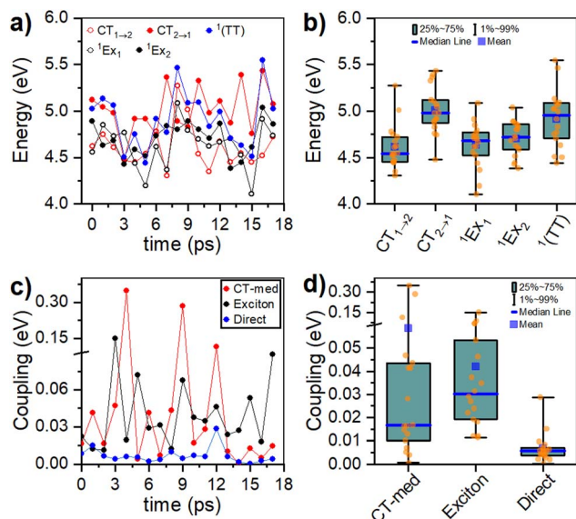
Fig. 7 (a) and (b) Fluctuations of diabatic state energies (in eV) and statistical dispersion parameters. CT_{1\rightarrow2} , CT_{2\rightarrow1} stand for charge-transfer states from monomer 1 to monomer 2, and from monomer 2 to monomer 1, respectively. Ex_1 and Ex_2 stand for local excited states localized on monomer 1 and monomer 2, respectively. {}^1(TT) stands for the correlated triplet-pair state. (c) and (d) Fluctuations of interstate couplings (in eV) computed along the AIMD dynamics of the lowest-energy PTC dimer and statistical dispersion parameters. Direct S_1/{}^1(TT) SF-coupling (blue); CT mediated SF-coupling (red); exciton coupling (black).
