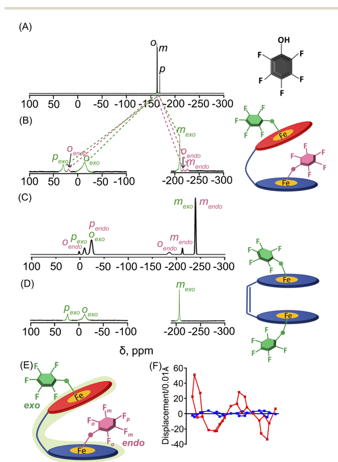
Fig. 4 19 F NMR spectra (at 298 K in C 6 D 6 ) of (A) free pentafluorophenol and (B) 2b . (C) DFT calculated 19 F NMR spectrum of 2b . (D) 19 F NMR spectrum (in CDCl 3 at 298 K) of the pentafluorophenolato analogue of the cis -ethene bridged diiron(III)porphyrin dimer ( exo-exo form, Scheme S1 † ). (E) Schematic representation of the exo-endo conformer upon pentafluorophenol binding. (F) Out-of-plane displacement of the porphyrin core atoms of 2b from the least-squares plane of the C 20 N 4 porphyrinato core. The horizontal axis represents the bond connectivity between atoms.
