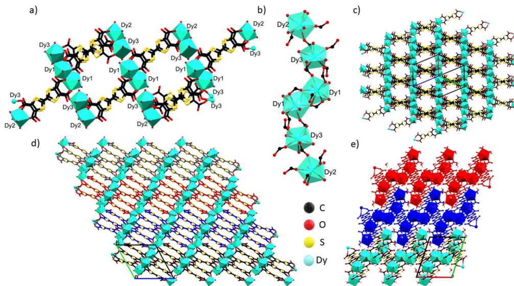
Fig. 2 (a) Crystal packing fragment highlighting the connectivity of the SBUs; (b) coordination environment in Dy_6 clusters that act as an SBU; (c) crystal packing along [111] ; (d) crystal packing along the a axis, C atoms from different layers are black, blue, red and grey; (e) crystal packing along the c axis, red and blue colored atoms belong to different layers. H atoms and uncoordinated water molecules are omitted for clarity.
