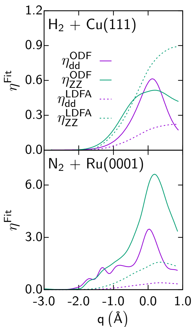
Figure 11. Diagonal elements of the friction tensor, \eta_{qq} (in \text{meV ps \AA}^{-2} ), are shown as a function of q ( d is the bond distance of the molecule, Z the distance of the molecule's center of mass to the surface) for the LDFA and the ODF approximations, as computed for \text{H}_2 + \text{Cu}(111)^{136} and \text{N}_2 + \text{Ru}(0001)^{61} . Data taken from Ref. 136 and Ref. 61 . This figure has been reproduced from Ref. 13 with permission from the Royal Society of Chemistry, copyright 2021.
