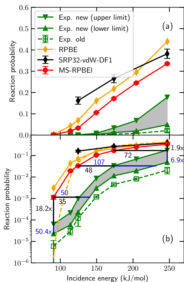
Figure 1. Sticking probabilities computed 45 for HCl + Au(111) with the MS-RPBEI meta-GGA DF 45 , the RPBE GGA DF 177 , and the SRP32-vdW1 DF featuring semi-local exchange and non-local correlation 46 are compared to experimental results, for normal incidence. The open green squares are the experimental sticking probabilities first published 286 , while the upper base and lower base triangles represent upper and lower bounds to the experimental S_0 obtained from an improved analysis of the experiments 45 . Panel a uses a linear and panel b a logarithmic scale for S_0 . In panel b results of QCT 177 (orange diamonds connected by solid orange line) as well as of QD 287 (orange dashed lines) calculations using the RPBE DF are presented. Figure taken from Ref. 45 ( https://doi.org/10.1021/acs.jpcc.0c03756 ). Further permission requests to be directed to the ACS.
