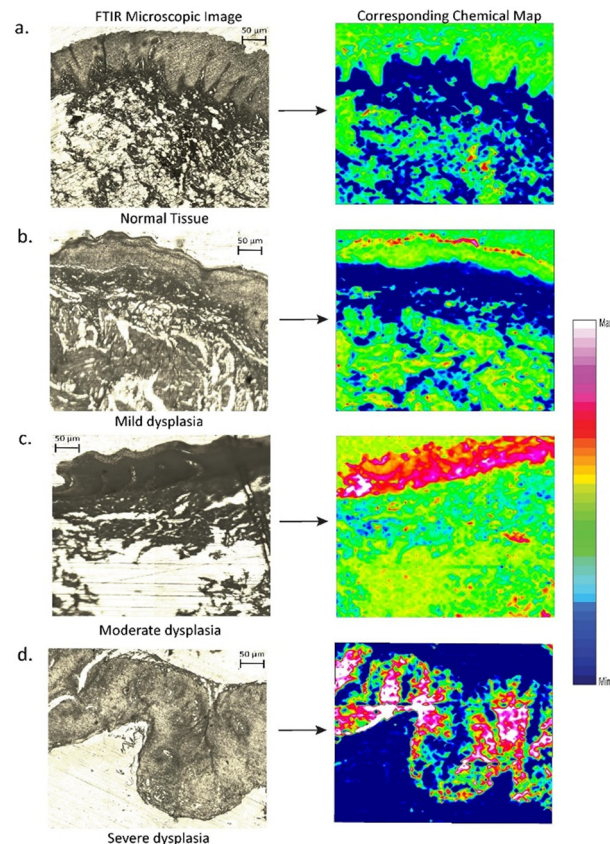
Fig. 6 Photographs of FTIR images with their corresponding chemical maps in the amide III absorption band (1340–1240 \text{cm}^{-1} ) for (a) normal tissue (b) mild dysplasia (c) moderate dysplasia and (d) severe dysplasia.
