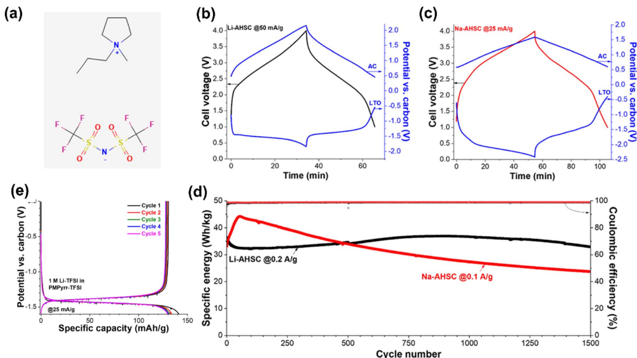
Fig. 3 (a) 1-Methyl-1-propylpyrrolidinium bis(trifluoromethanesulfonyl)imide ( \text{Pyr}_{13}\text{TFSI} ) ionic liquid molecular structure. Voltage profiles of (b) Li-based supercapacities cycled at 50 \text{ mA g}^{-1} and (c) Na-based supercapacities cycled at 25 \text{ mA g}^{-1} , including potential development at the negatode ( \text{Li}_4\text{Ti}_5\text{O}_{12} ) and positrode (activated carbon). (d) The cycling stability of Li-based supercapacities cycled at 0.2 \text{ A g}^{-1} , and Na-based supercapacities cycled at 0.1 \text{ A g}^{-1} over 1500 cycles between 1 V and 4 V cell voltage. (e) Comparison of the first 5 galvanostatic cycles in 1 M LiTFSI in \text{Pyr}_{13}\text{TFSI} electrolyte at 25 \text{ mA g}^{-1} . 32 (Reprinted from ref. 32 with permission from Rightslink).
